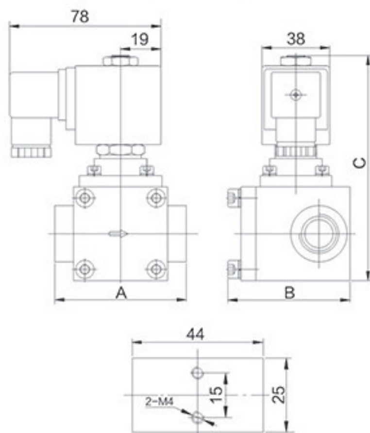
UYSE-010~040底面安装孔
